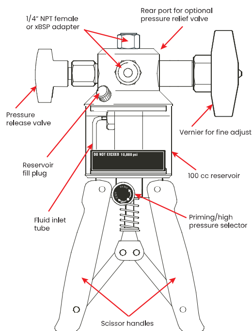
PV212-X components
